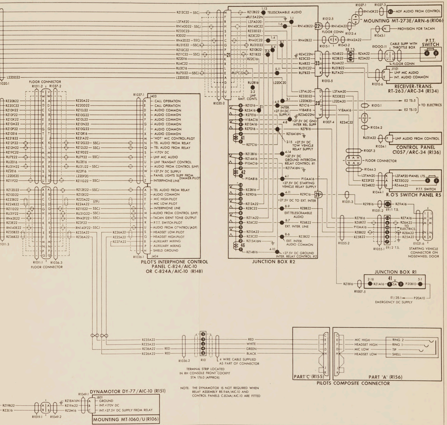
FIG. 3 AN/AIC-10 INTERPHONE SYSTEM
