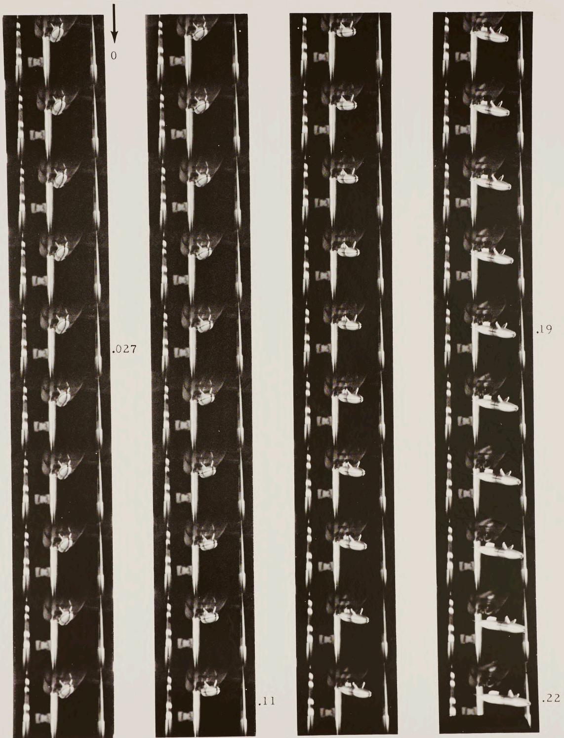
FIG. 6 (a) FRONT VIEW RUN NO. 13 - SEA LEVEL, M = .50 , \mathcal{L} = 2.3^\circ TANK EMPTY, \psi = -5^\circ FILM SPEED 696 FRAMES PER SECOND.
