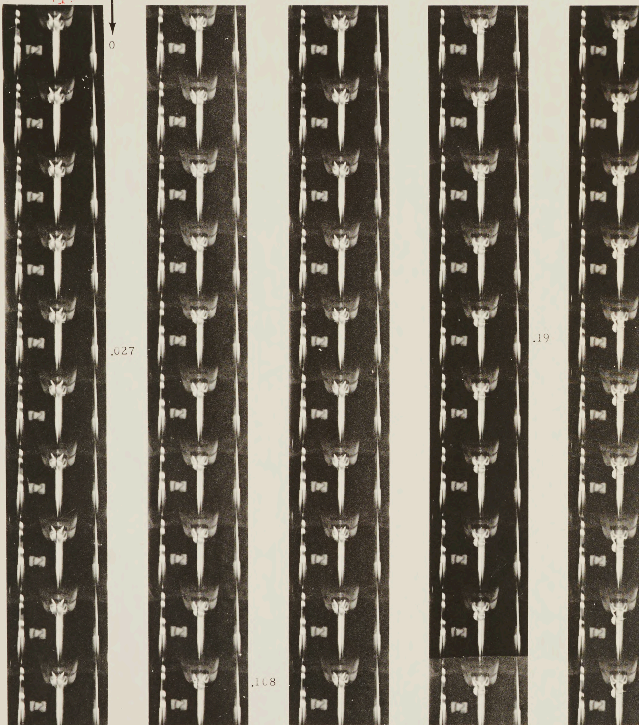
FIG. 5 (a) FRONT VIEW RUN NO. 12 - 40,000 FT., M = .85 , \alpha = 4.4^\circ TANK FULL, \psi = 0 FILM SPEED 700 FRAMES PER SECOND.
