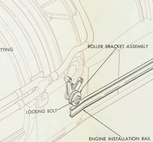
METHOD OF ENGINE ATTACHMENT AND SUSPENSION, ARROW 2/IROQUOIS
