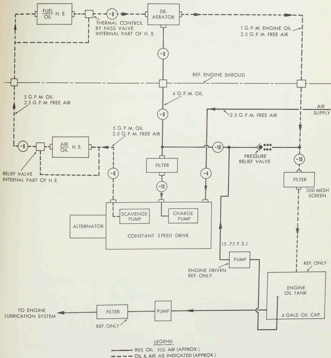
ARROW 2 CONSTANT SPEED DRIVE INTEGRATED OIL SYSTEM
