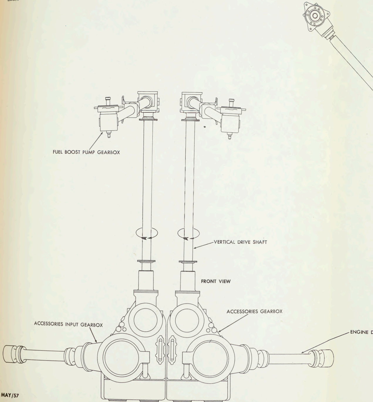
FIG. 5 ACCESSORIES GEARBOX
