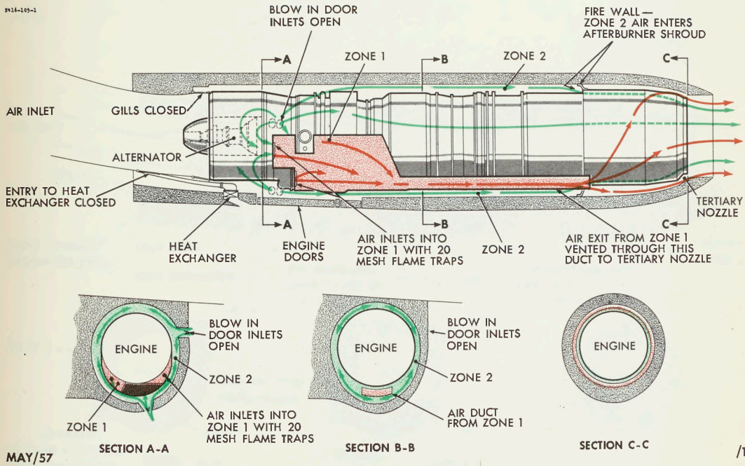
FIG. 3 ENGINE COOLING-STATIC CASE AND UP TO APPROXIMATELY MACH .50
