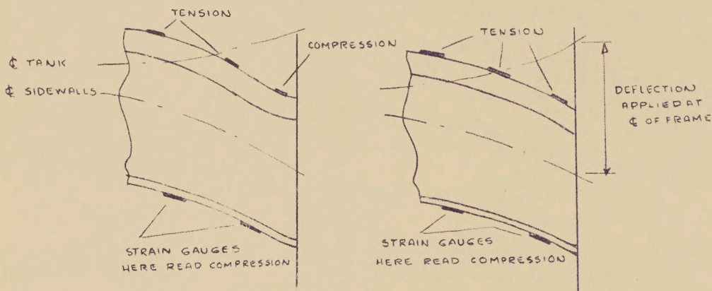
(b) LONGERON FIXITY DESTROYED
