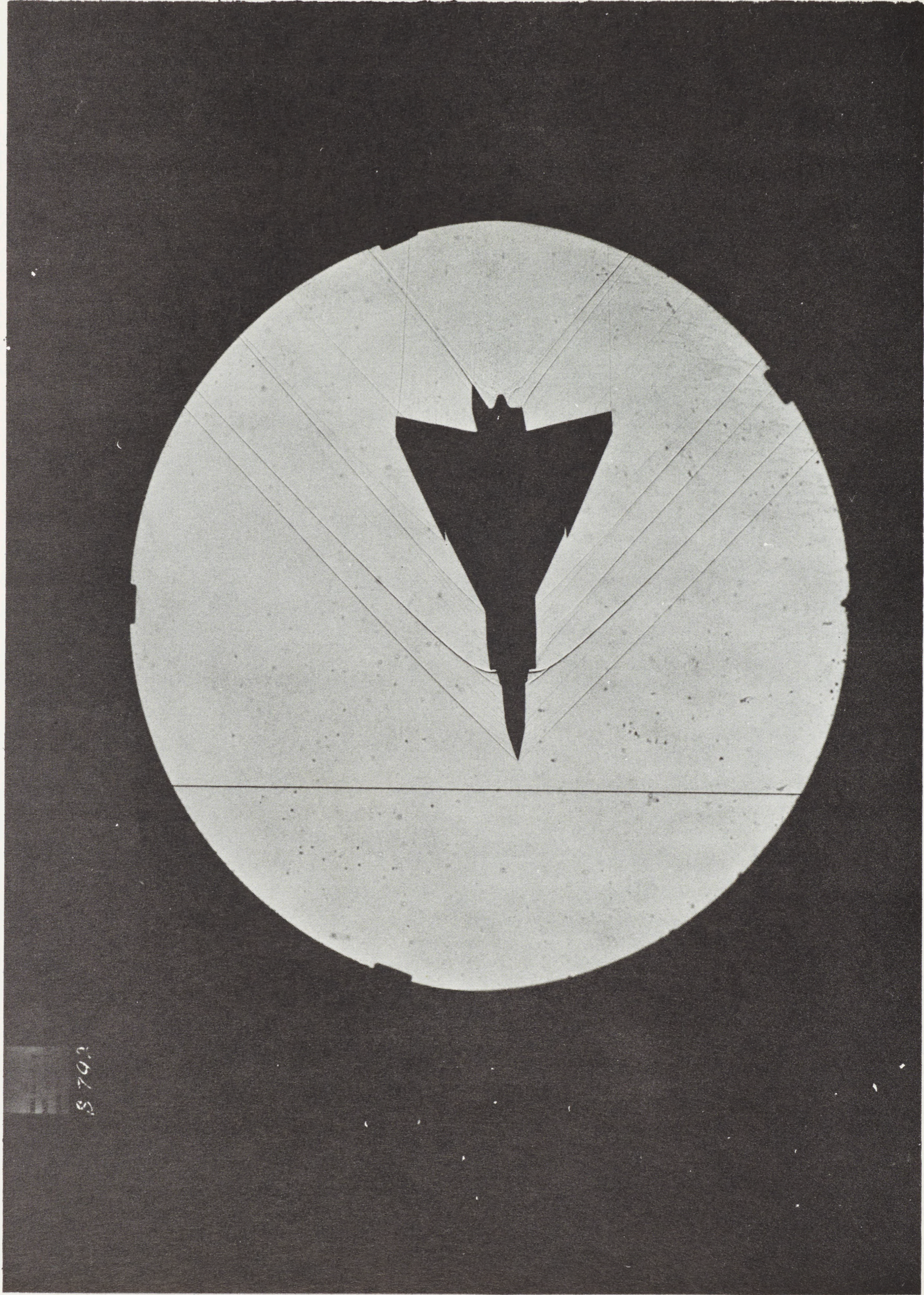
SHADOWGRAPH OF MODEL 10-19
