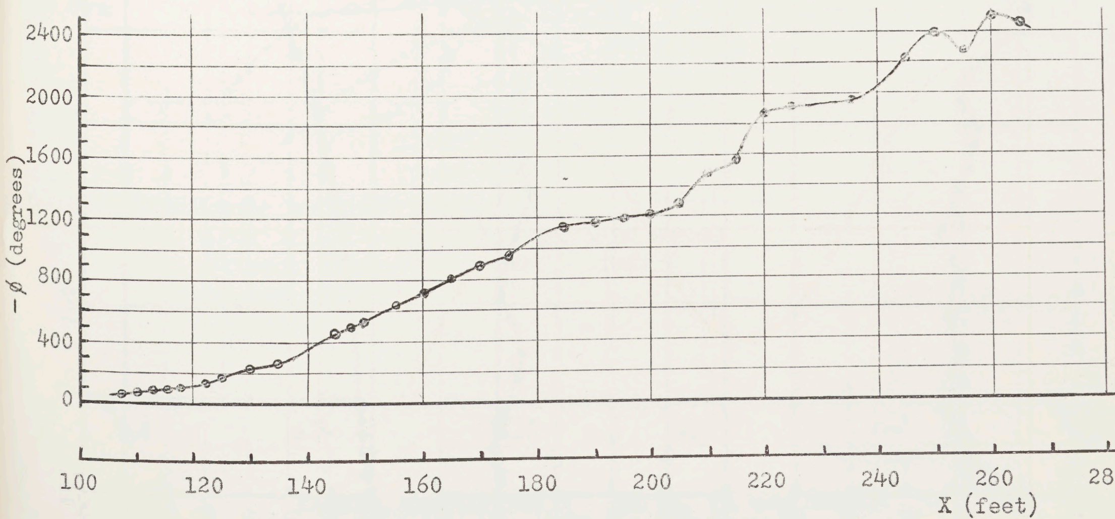
TEST RECORD FOR MODEL 10-16 FIGURE 8c
