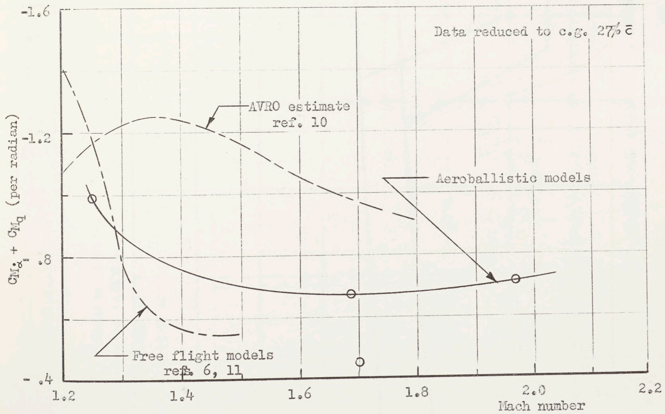
LONGITUDINAL DERIVATIVES C_{M_\alpha} AND (C_{M_\alpha} + C_{M_q}) VS. MACH NUMBER
