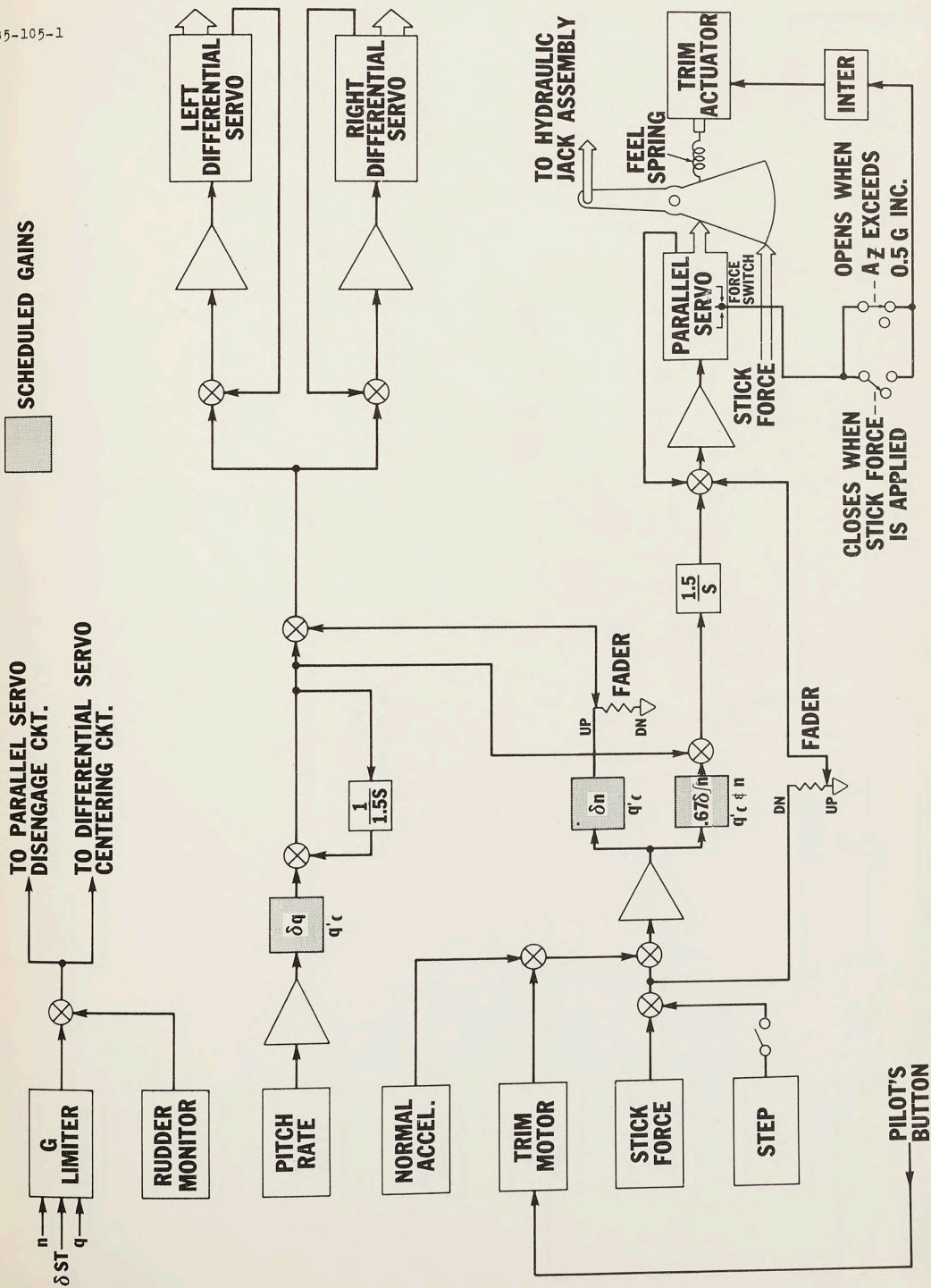
FIG. 4 MH-64 DAMPER, PITCH AXIS, ENGAGE, GEAR UP
