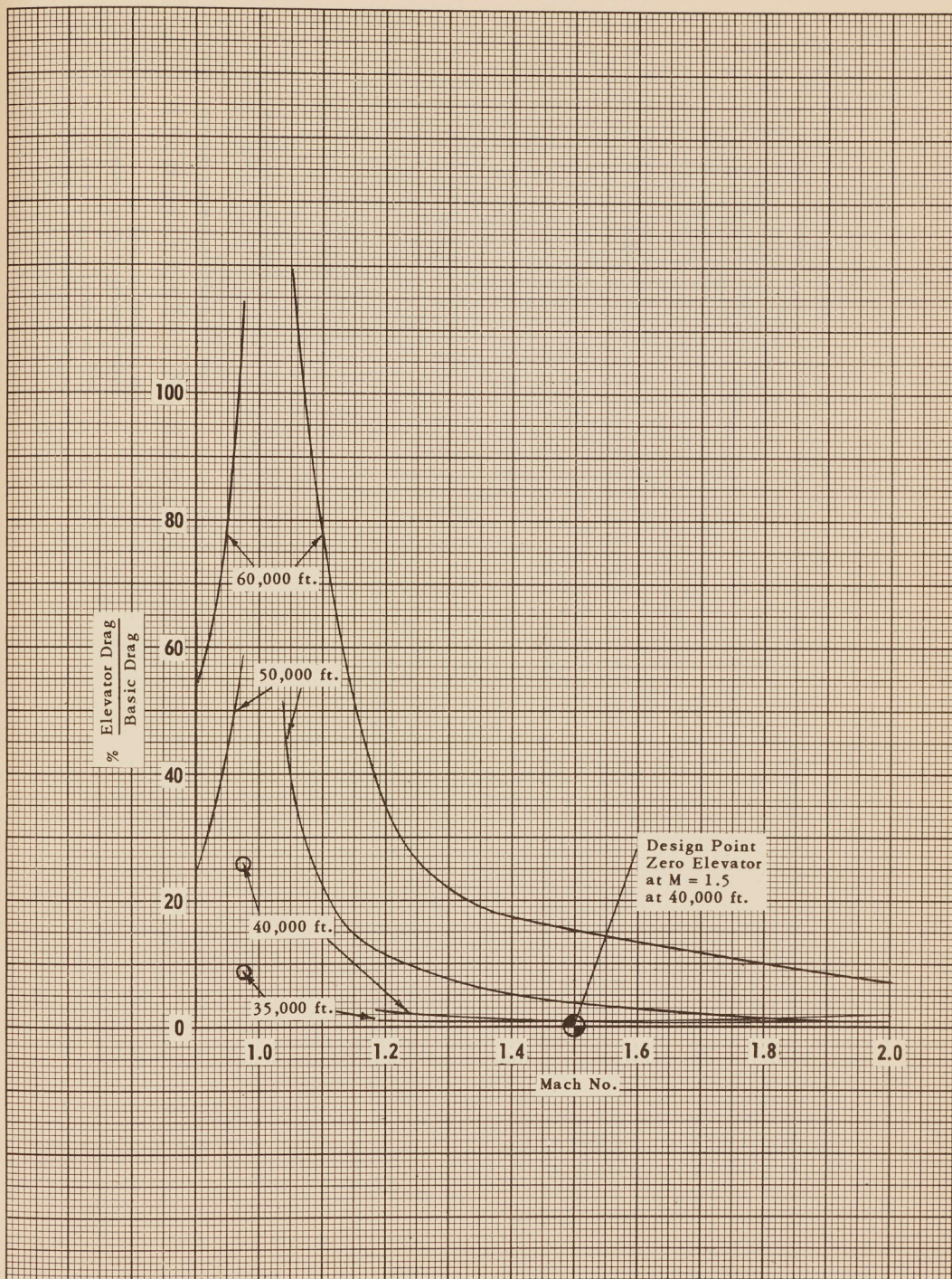
Fig. 5 0.5% Camber - % Elevator Drag Basic Drag
