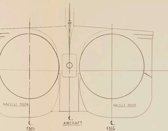
END VIEW LOOKING FWD. 1/8 SCALE
