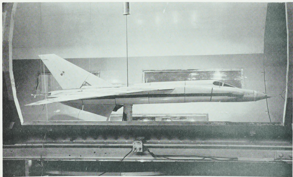
1/10TH SCALE FLUTTER MODEL
