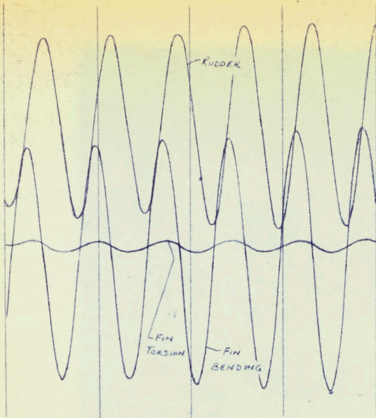
COMPONENT TEST FREE RUDDER 9.9 CPS - FULL SCALE 400 FT/SEC - FULL SCALE
