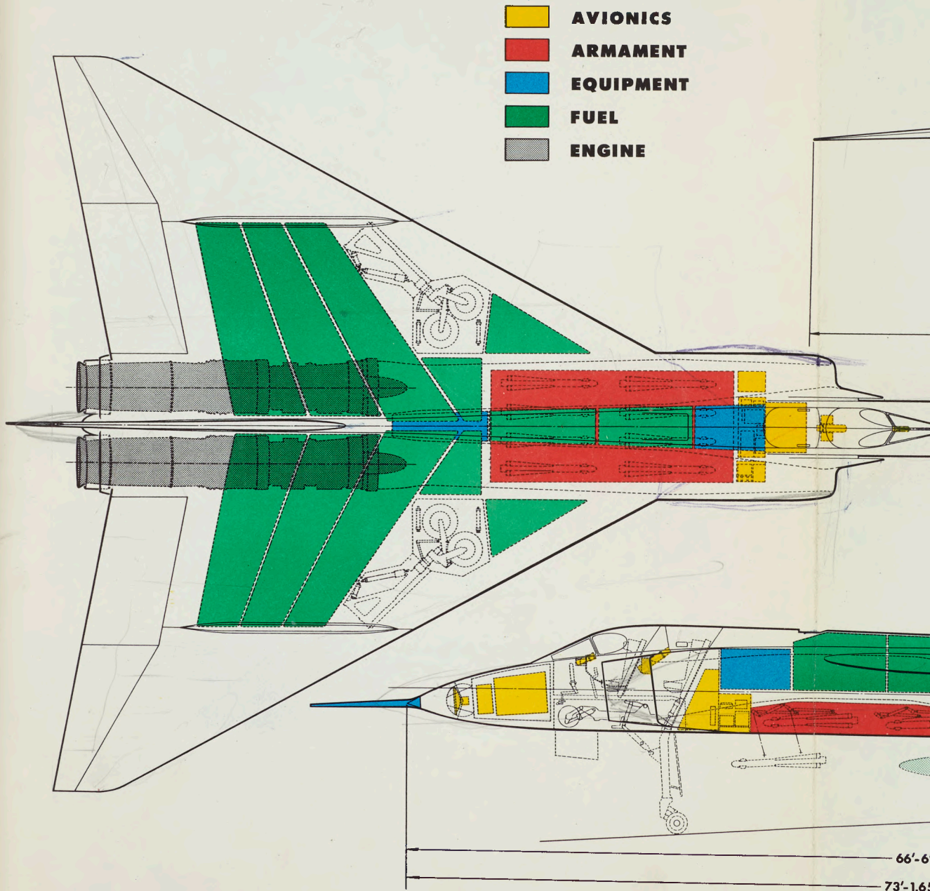
FIG. 1 3 VIEW GENERAL ARRANGEMENT
