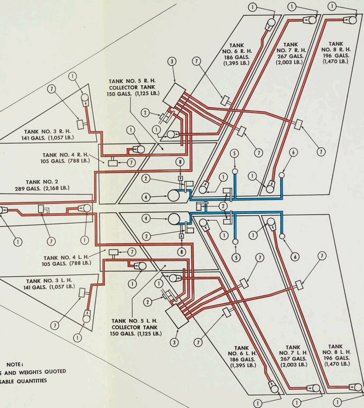
FUEL SYSTEM - DIAGRAMMATIC OF FUEL FEED AND TRANSFER
