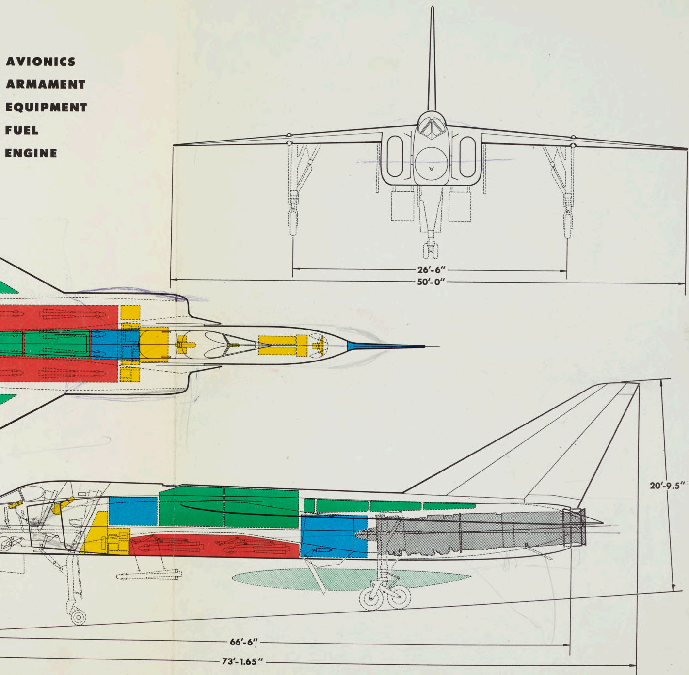
FIG. 1 3 VIEW GENERAL ARRANGEMENT
