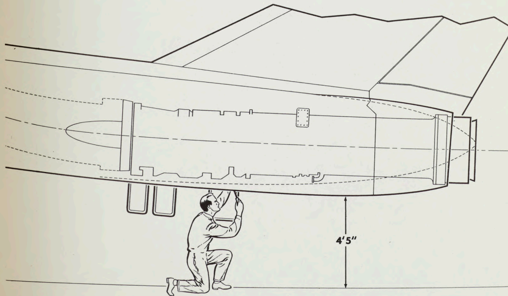
ENGINE SERVICING
