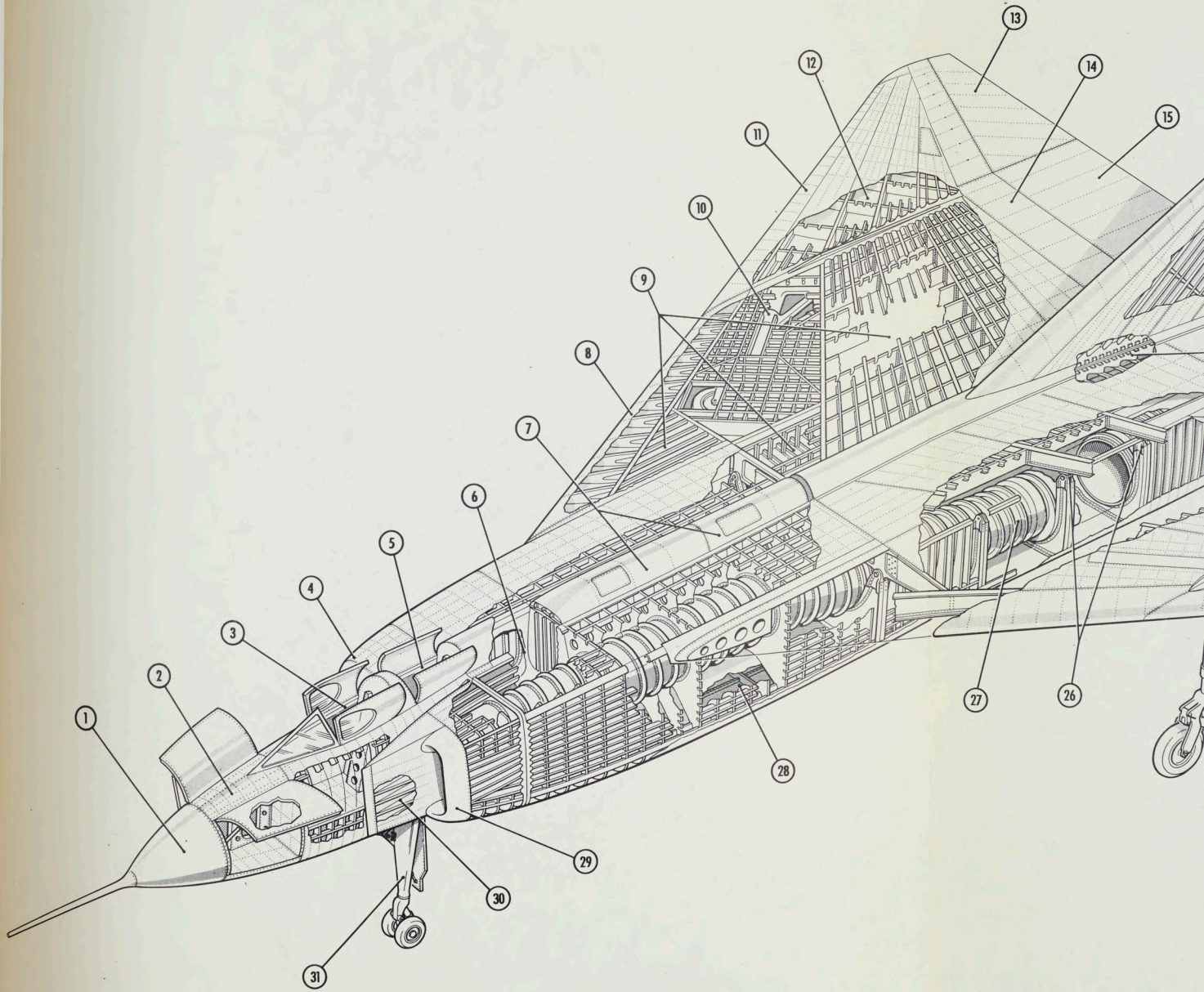
FIG. 27 STRUCTURE ARRANGEMENT
