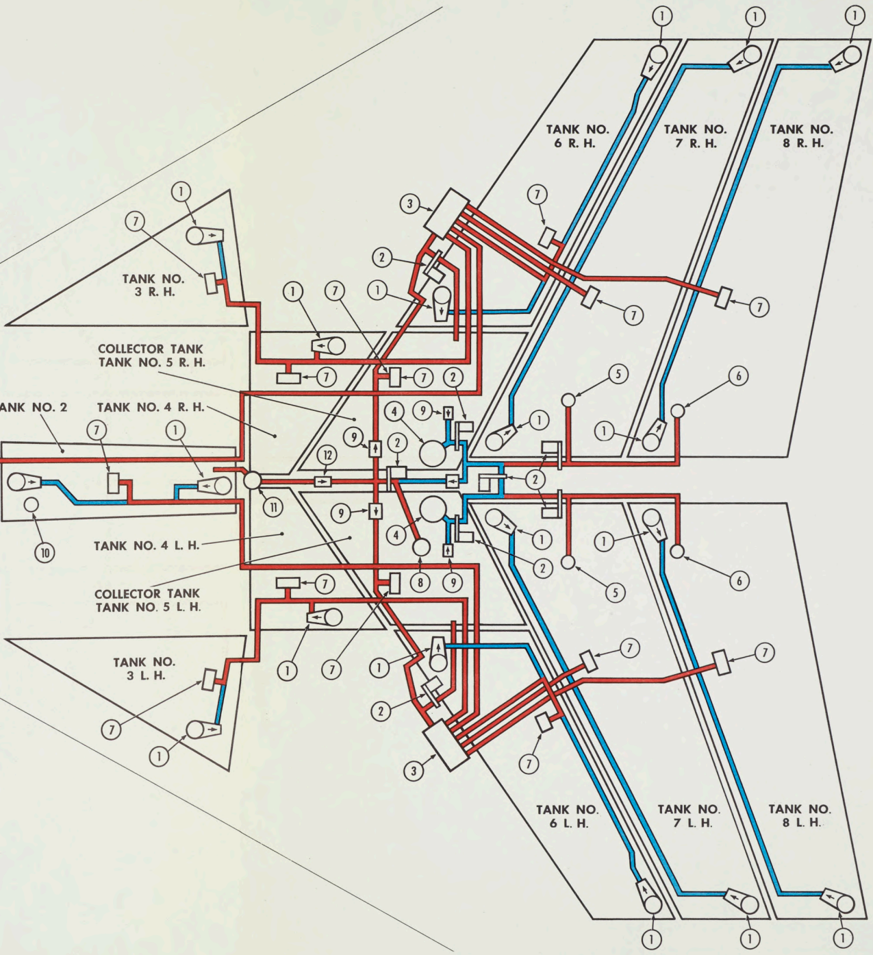
FUEL SYSTEM - DIAGRAMMATIC OF REFUELLING AND DEFUELLING
