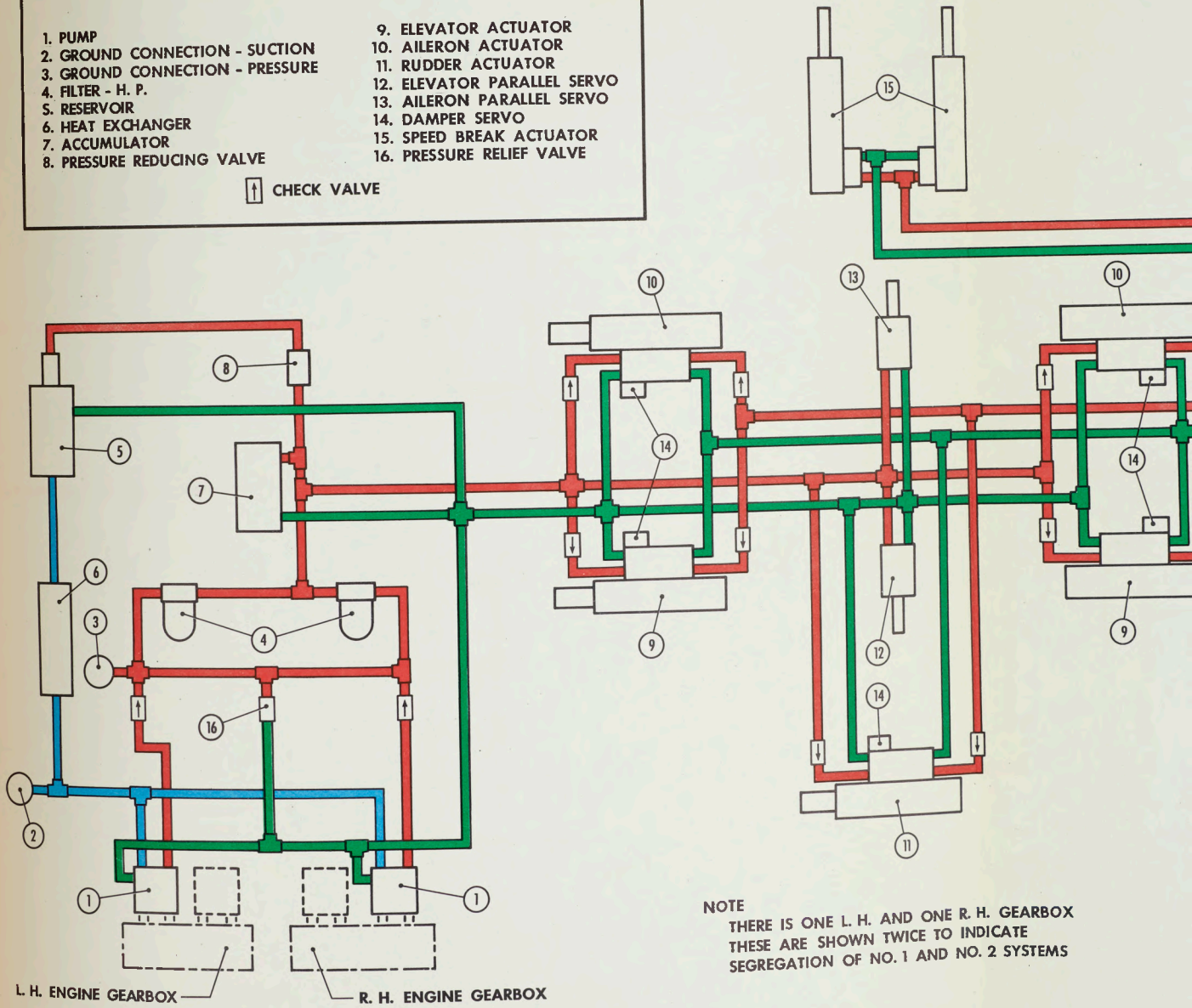
FLYING CONTROLS NO. 1 SYSTEM
