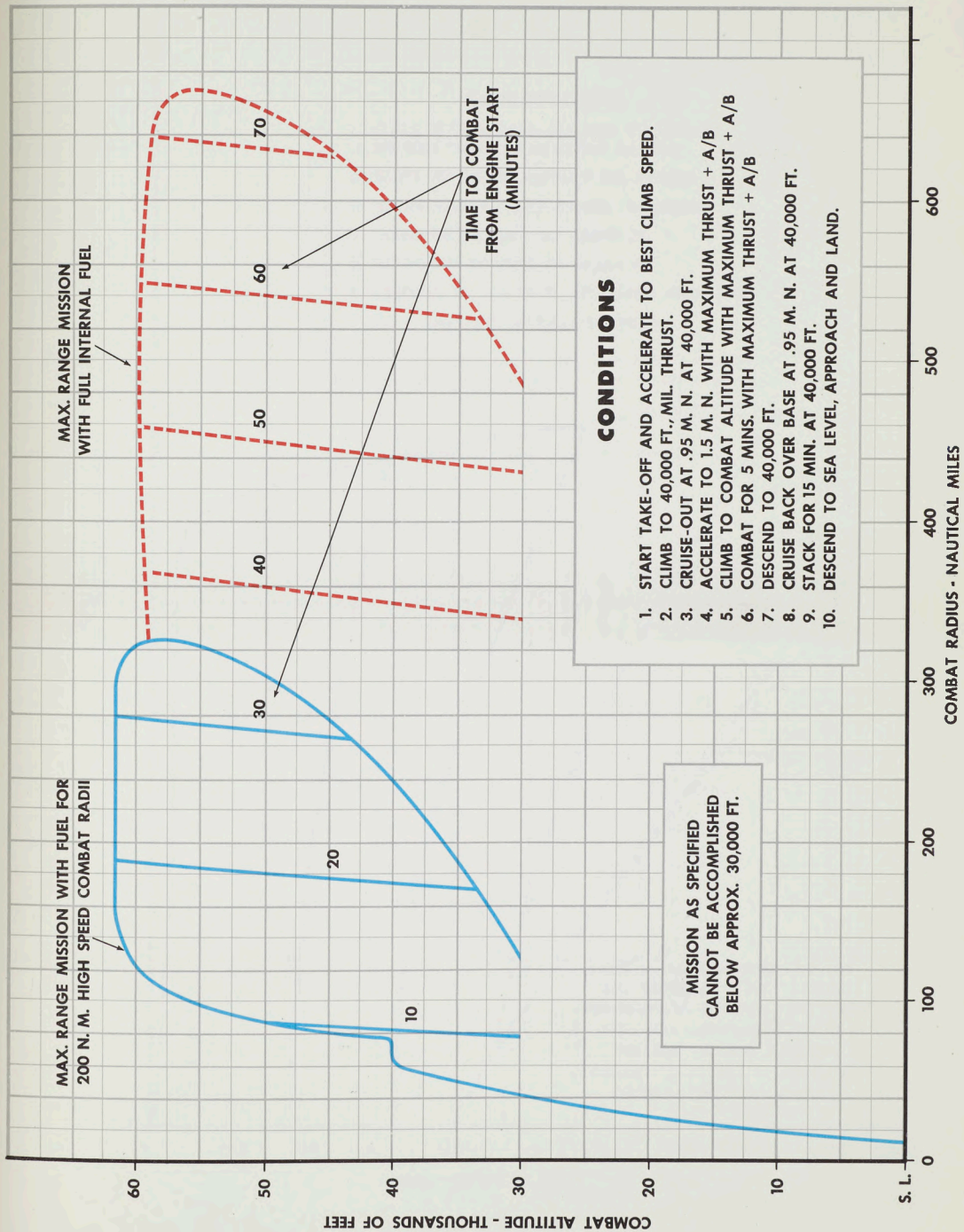
FIG. 12 MAXIMUM RANGE MISSION
