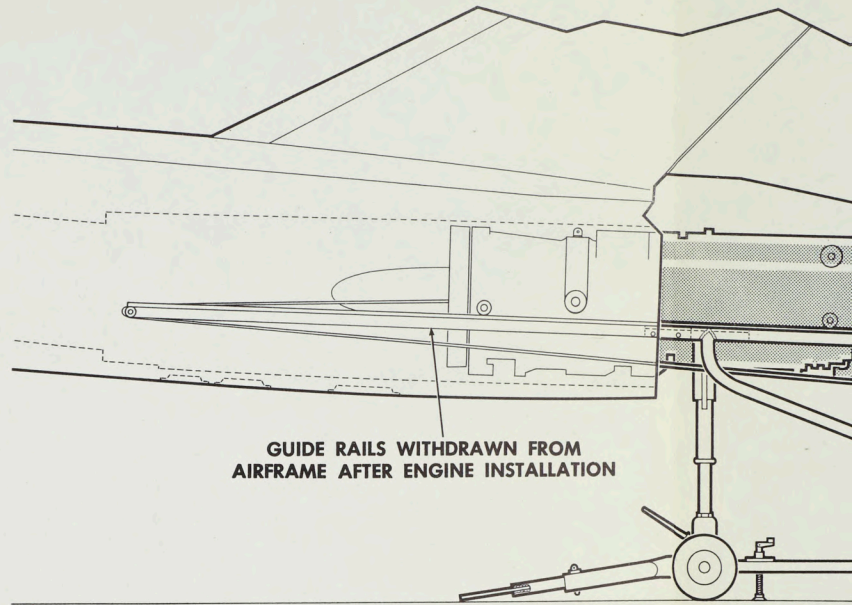
ENGINE INSTALLATION AND REM
