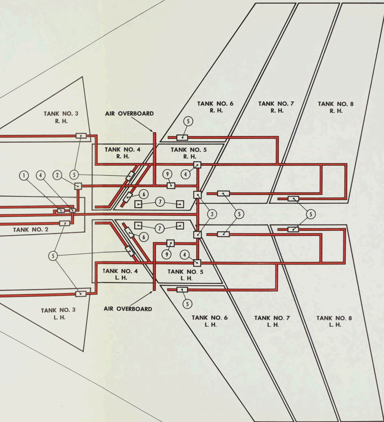
SYSTEM - DIAGRAMMATIC OF FUEL PRESSURIZATION
