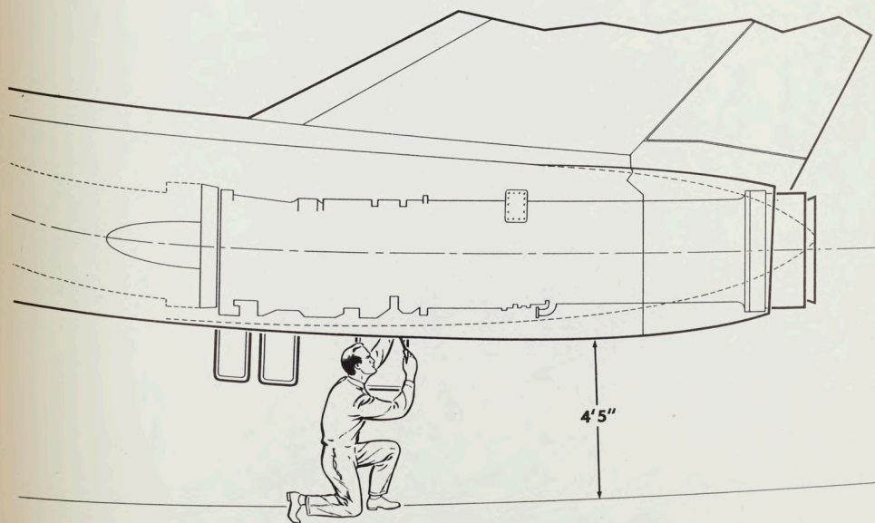
FIG. 28 ENGINE INSTALLATION AND REMOVAL
