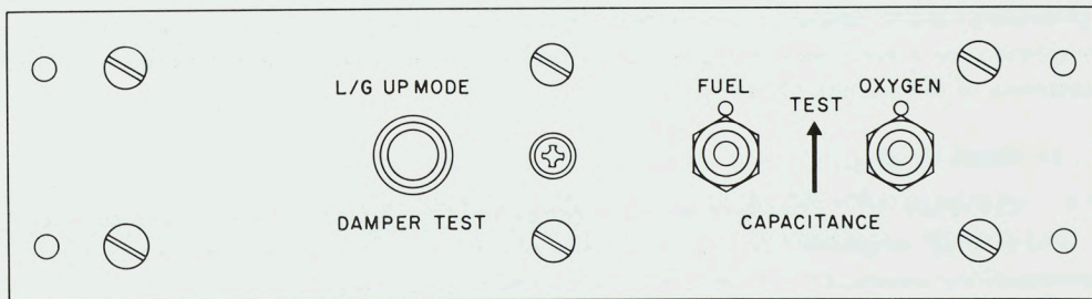
Figure 44. Fuel and Oxygen Test Panel
