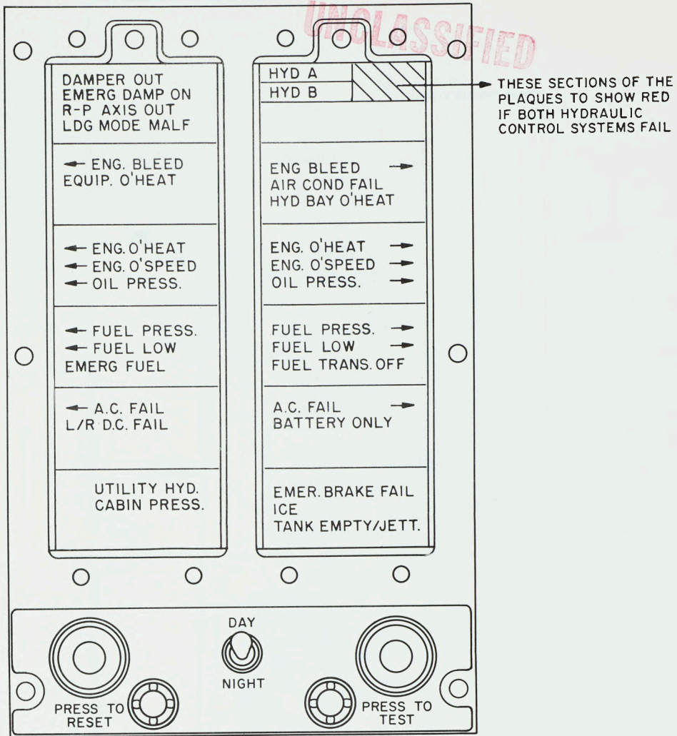
Figure 37. Warning Panel
