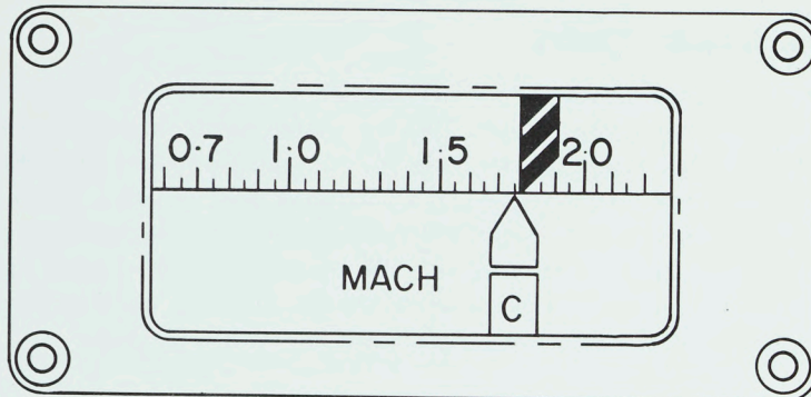
Figure 11. Mach Indicator
