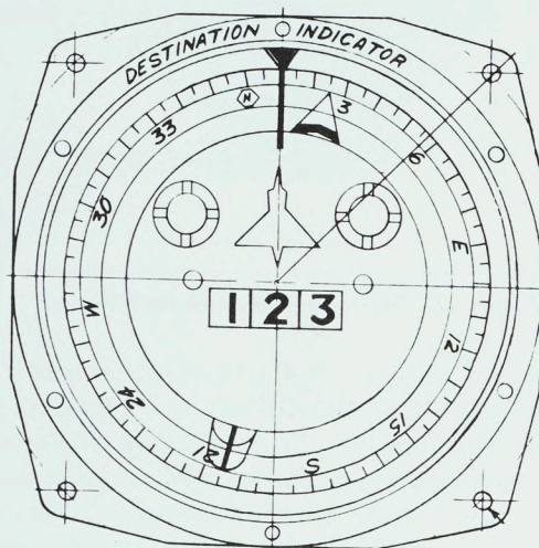
Figure 13. Destination Indicator
