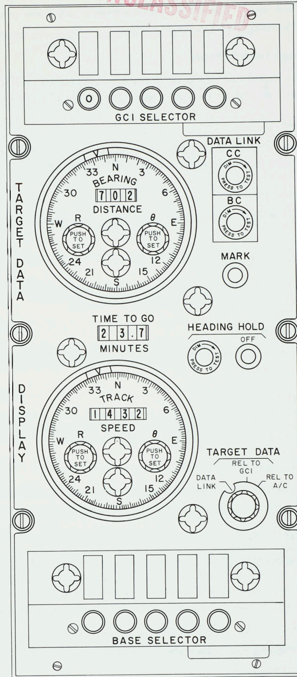
Figure 57. Target-Data Display
