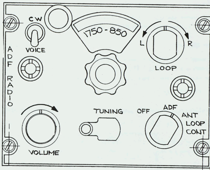
Figure 31. ARN-6 Control Panel
