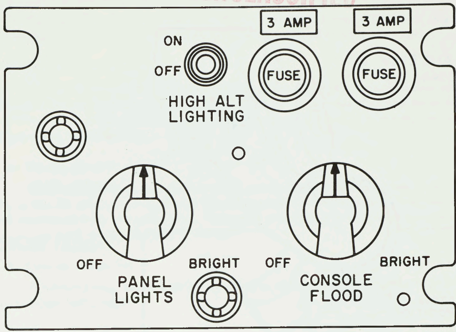
Figure 62. Observer's Panel and Console Lights Control
