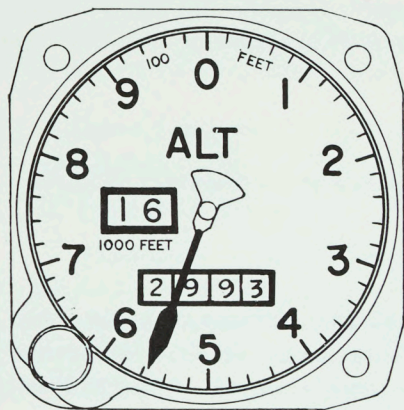
Figure 15. Altimeter
