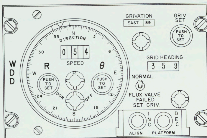
Figure 56. Wind-Data Display
