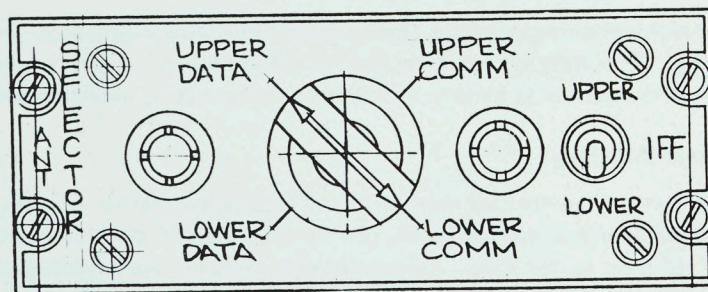
Figure 54. Antenna-Duplexer Control Panel
