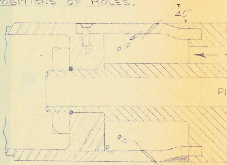
2 PART VIEWS SHOWING POSITIONS OF HOLES.
