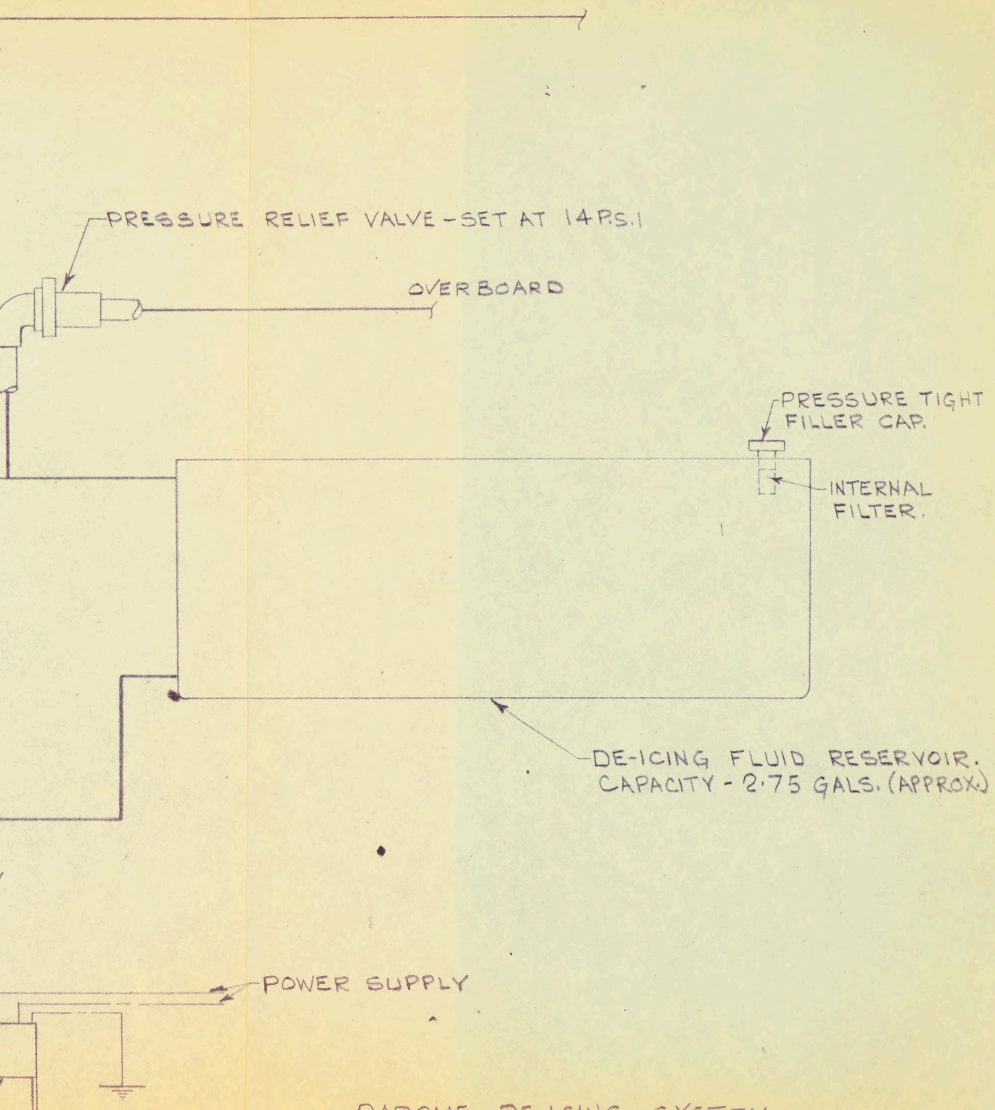
RADOME DE-ICING SYSTEM.
