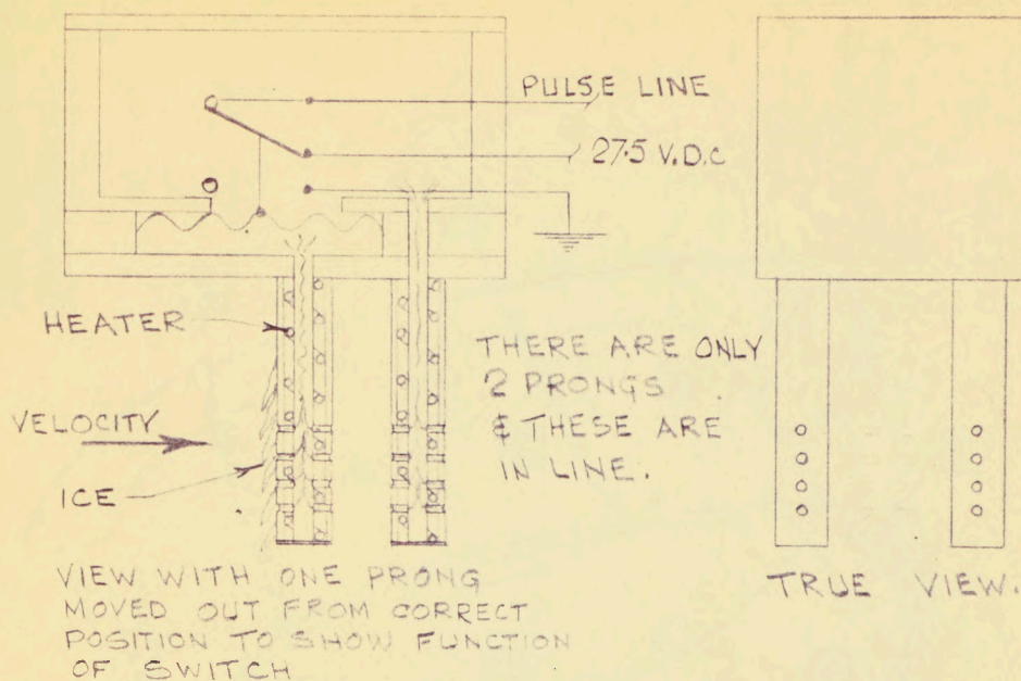
ICE DETECTOR IN ICED CONDITION
