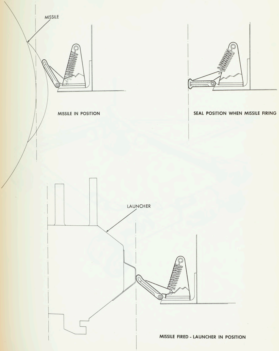
FIG. 9 MISSILE SEALS
